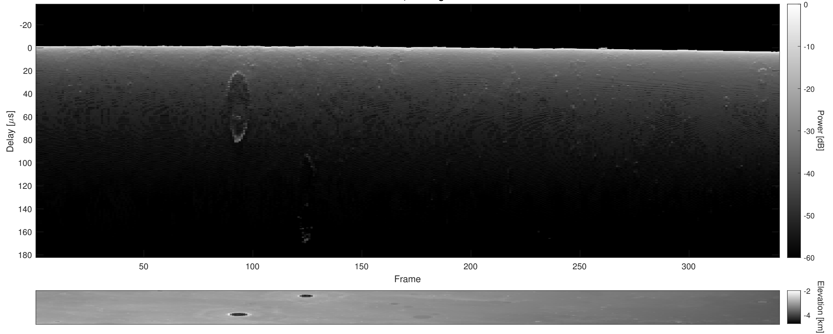
Orbit 16046, Cluttergram
