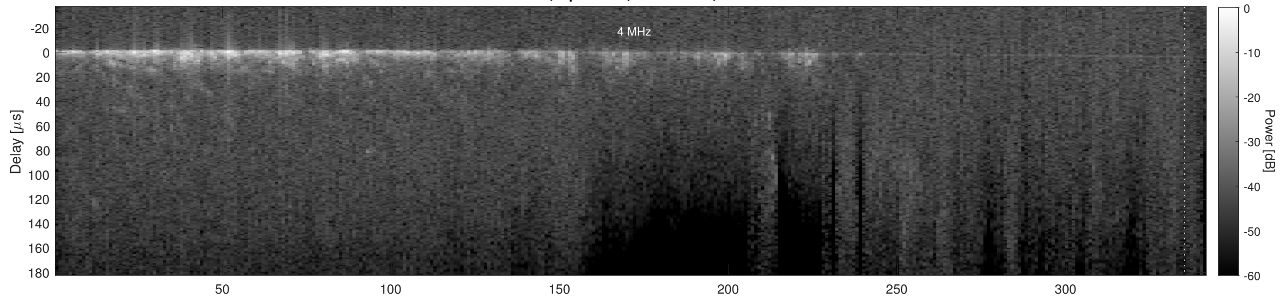
Orbit 16046, Cluttergram
