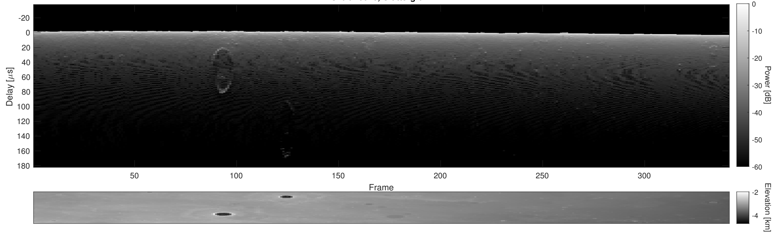
Orbit 16046, Cluttergram
