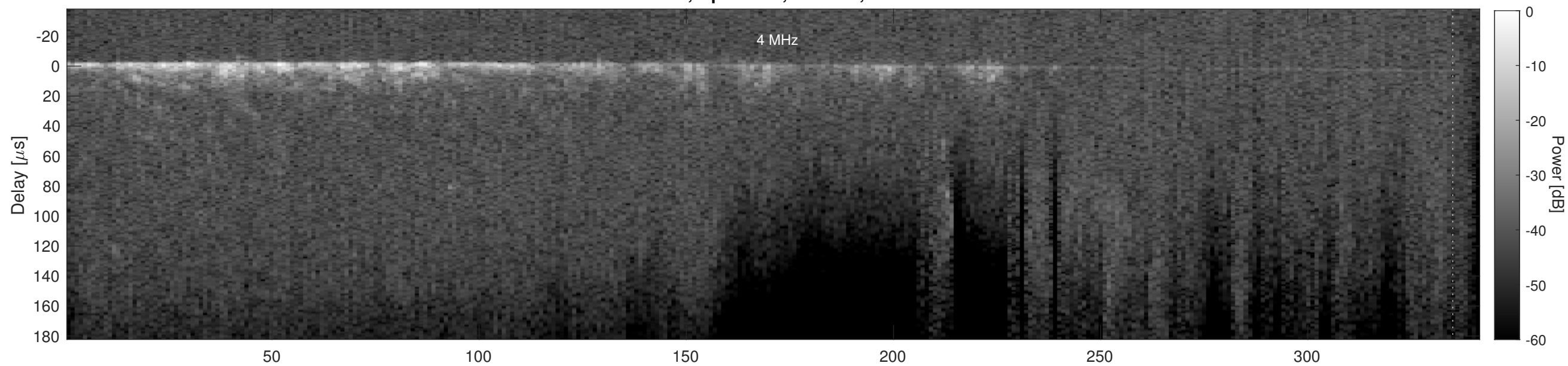
Orbit 16046, Cluttergram
