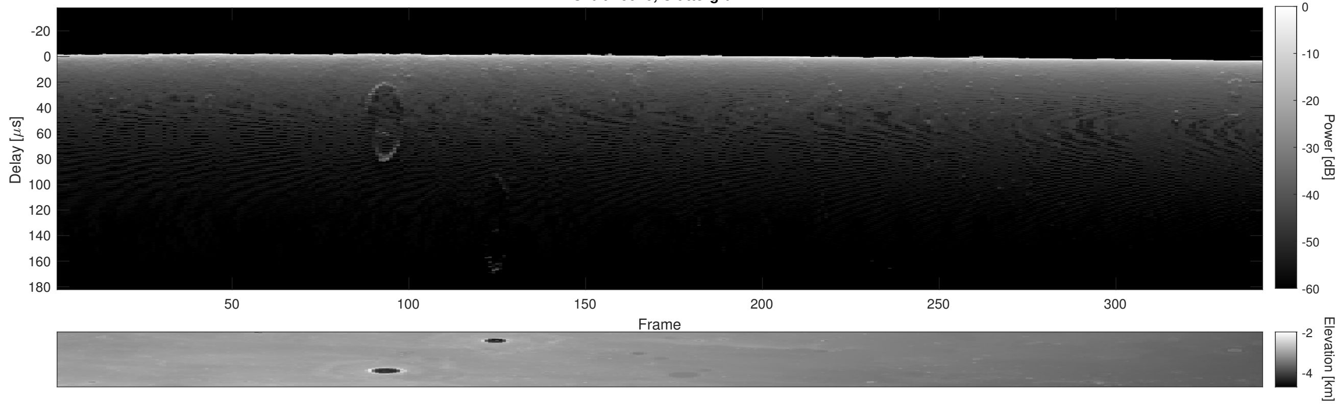
Orbit 16046, Cluttergram
