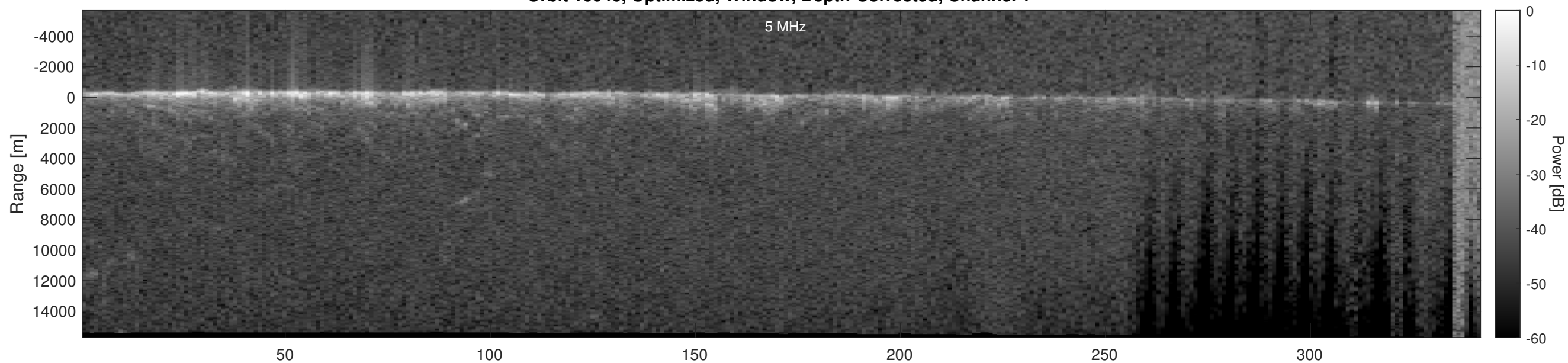
Orbit 16046, Optimized, Window, Depth-Corrected, Channel 2
