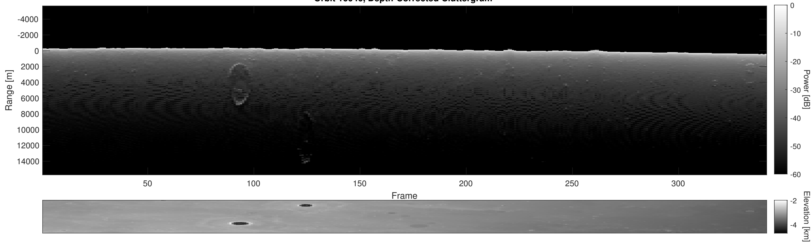
Orbit 16046, Depth-Corrected Cluttergram
