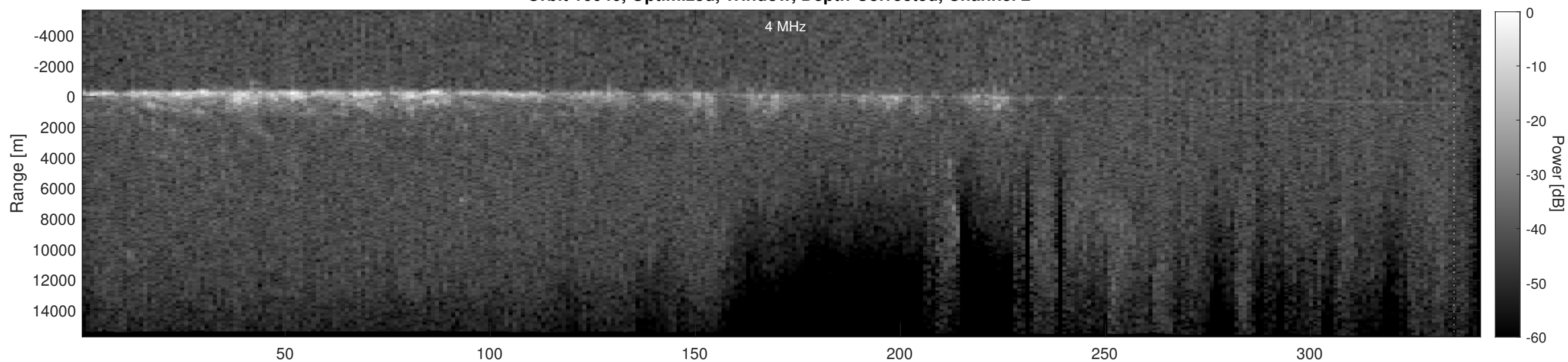
Orbit 16046, Depth-Corrected Cluttergram
