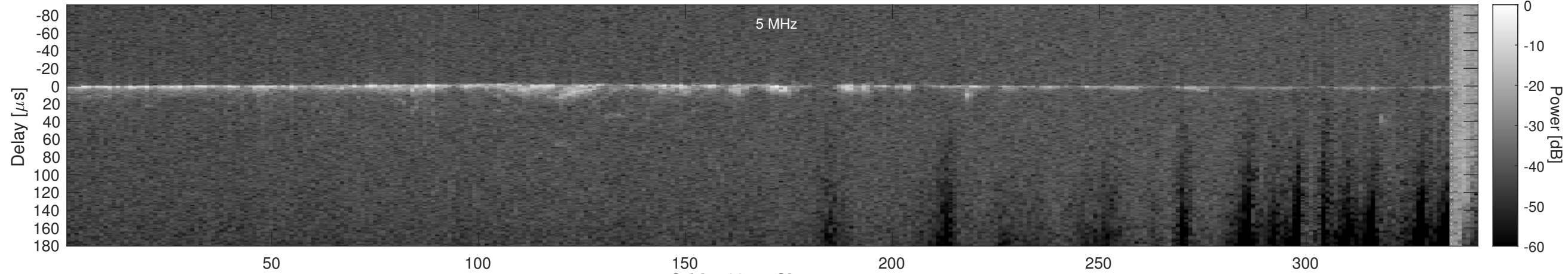
Orbit 16047, Cluttergram
