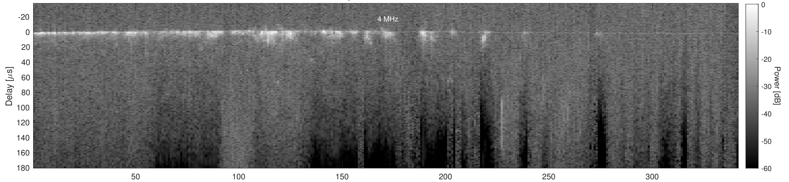
Orbit 16047, Cluttergram
