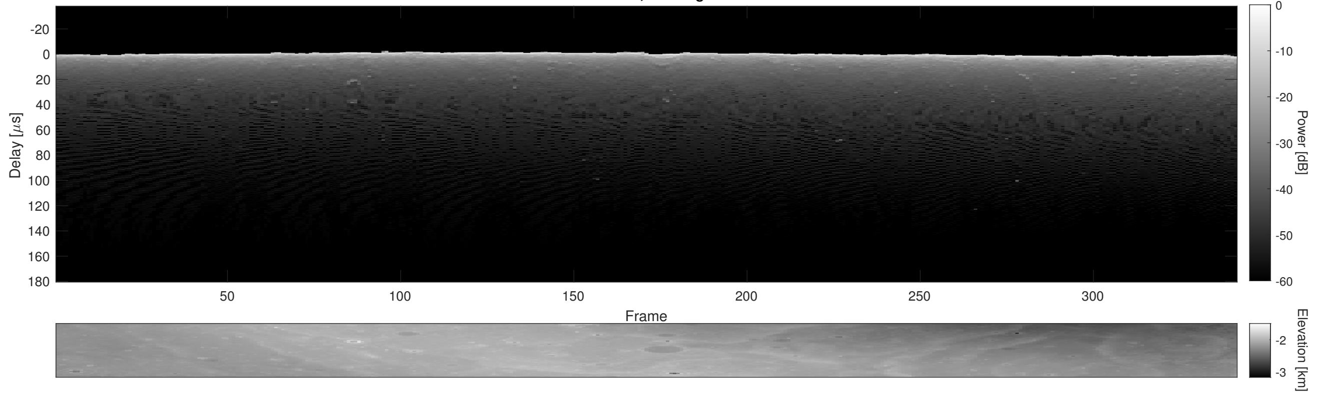
Orbit 16047, Cluttergram
