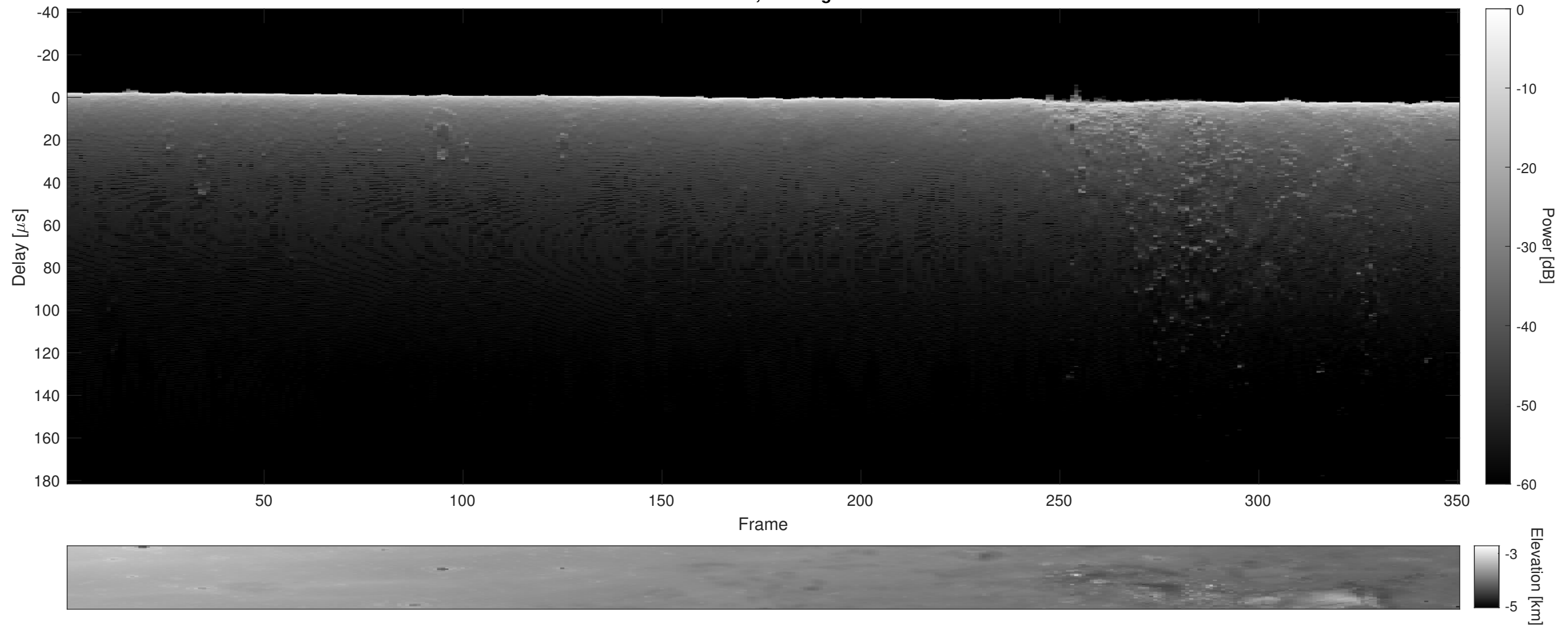
Orbit 16048, Cluttergram
