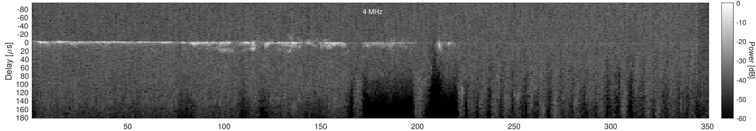
Orbit 16048, Cluttergram
