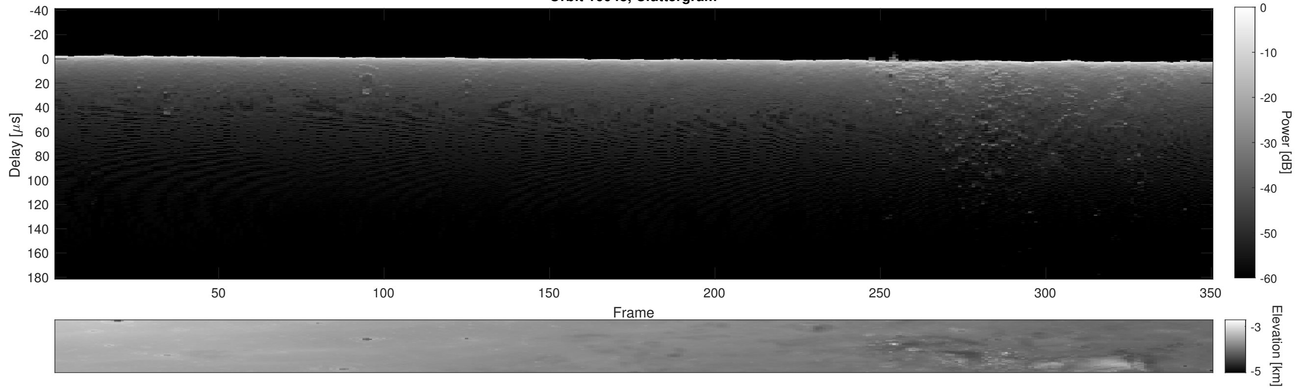
Orbit 16048, Cluttergram
