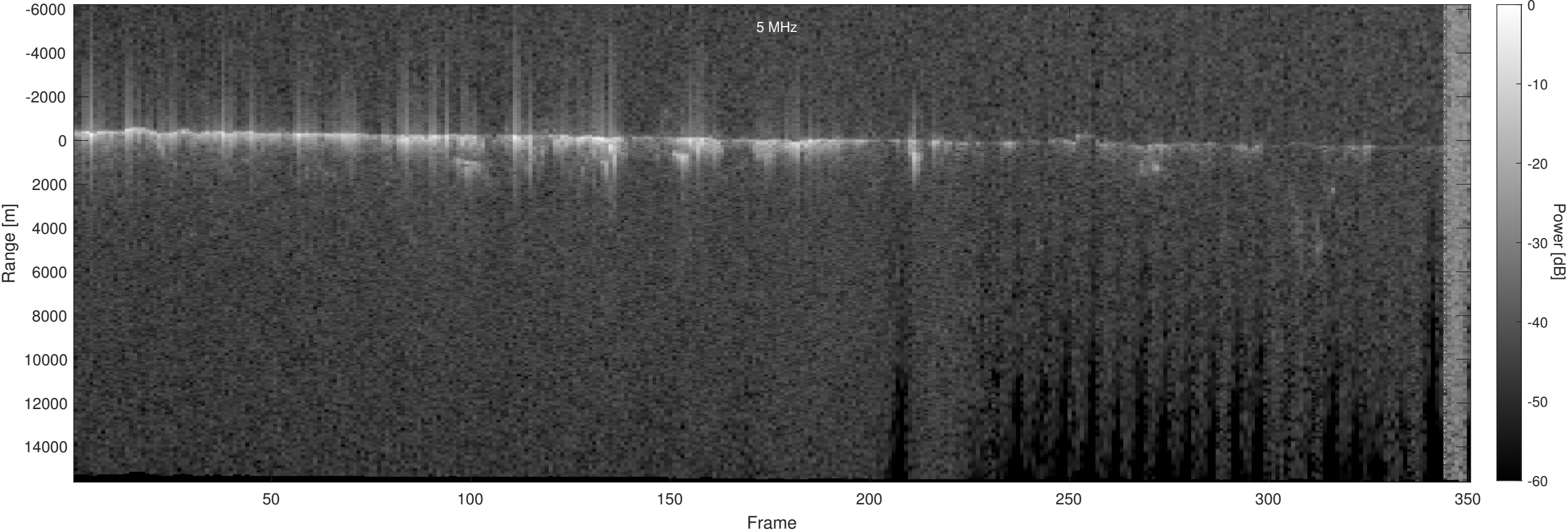
Orbit 16048, Optimized, No Window, Depth-Corrected, Channel 2
