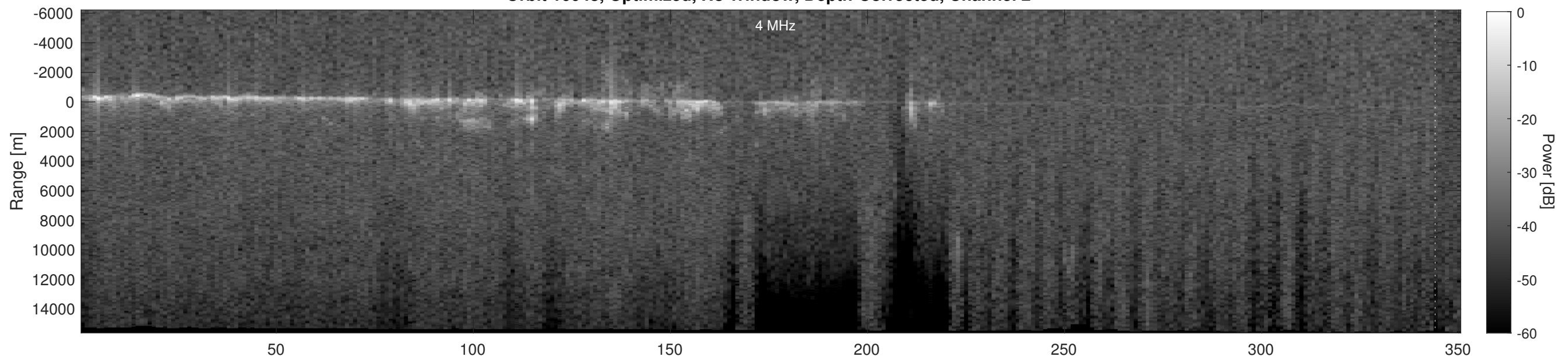
Orbit 16048, Depth-Corrected Cluttergram
