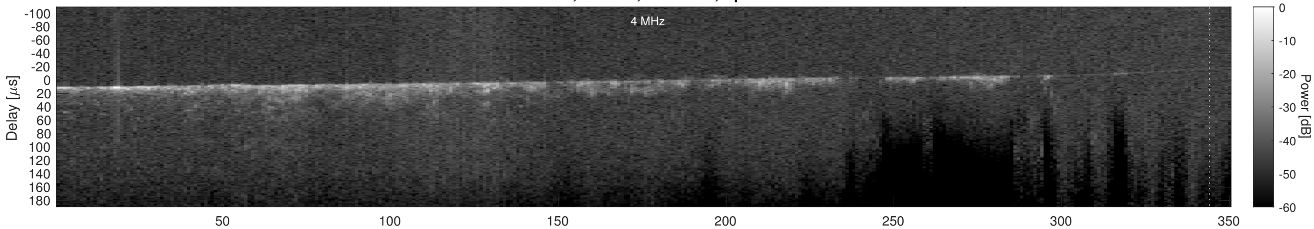
Orbit 16049, Cluttergram
