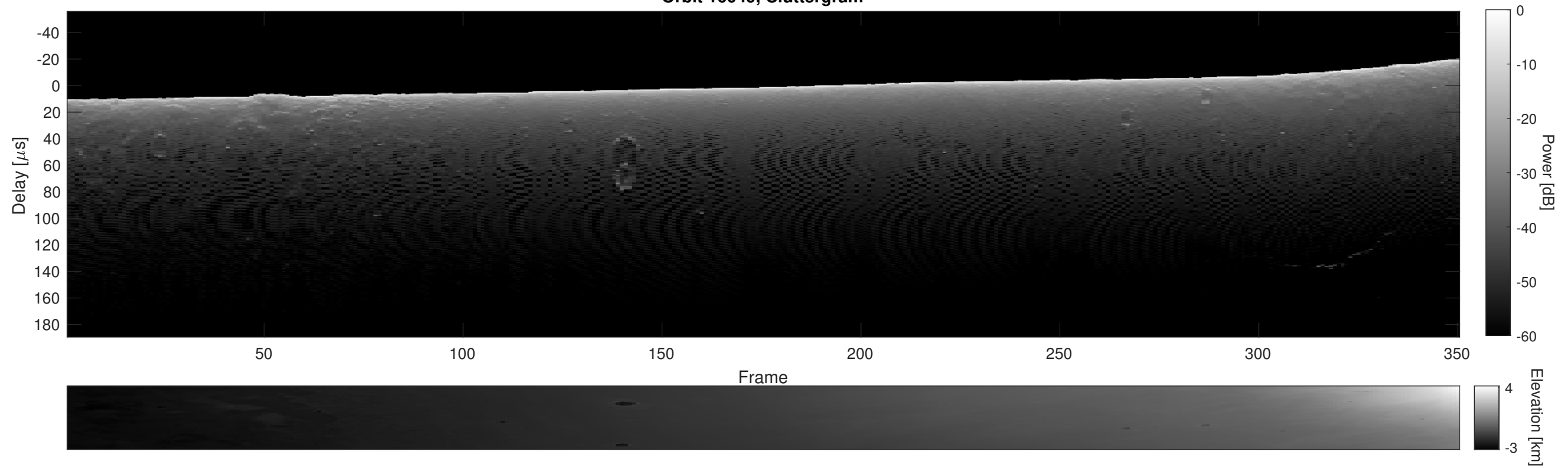
Orbit 16049, Cluttergram
