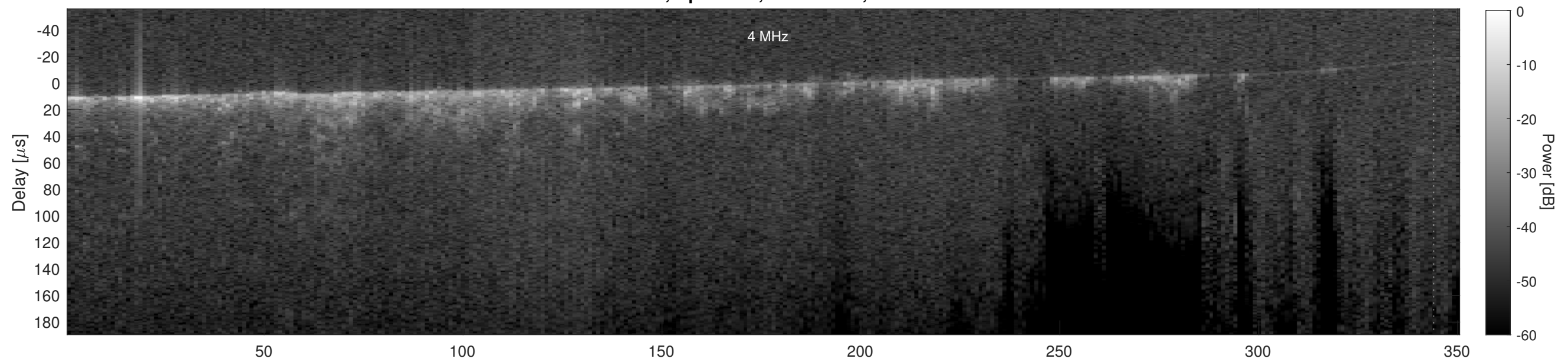
Orbit 16049, Cluttergram
