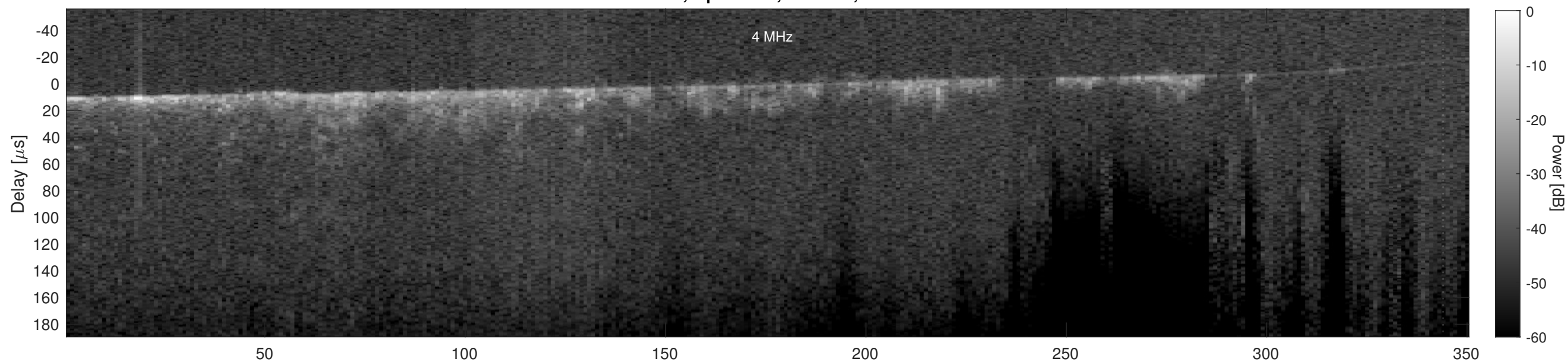
Orbit 16049, Cluttergram
