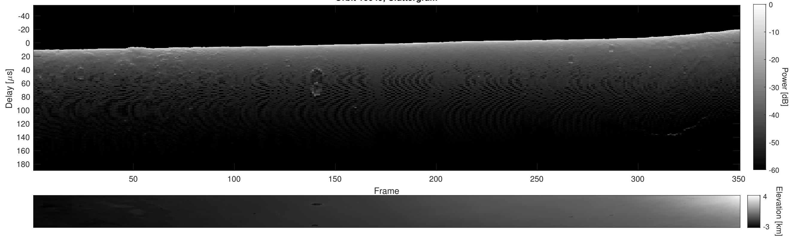
Orbit 16049, Cluttergram
