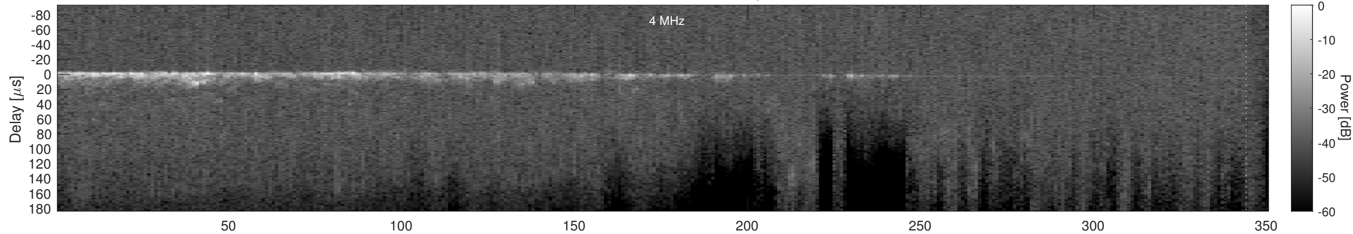
Orbit 16050, Cluttergram
