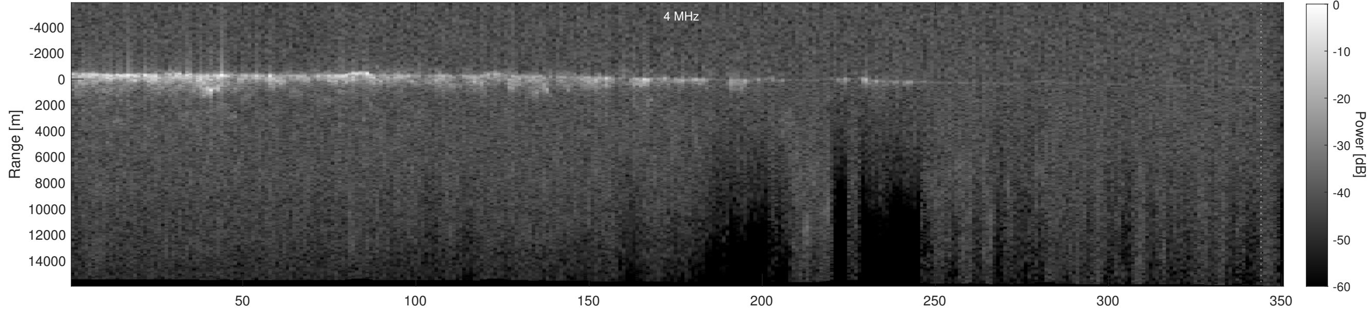
Orbit 16050, Depth-Corrected Cluttergram
