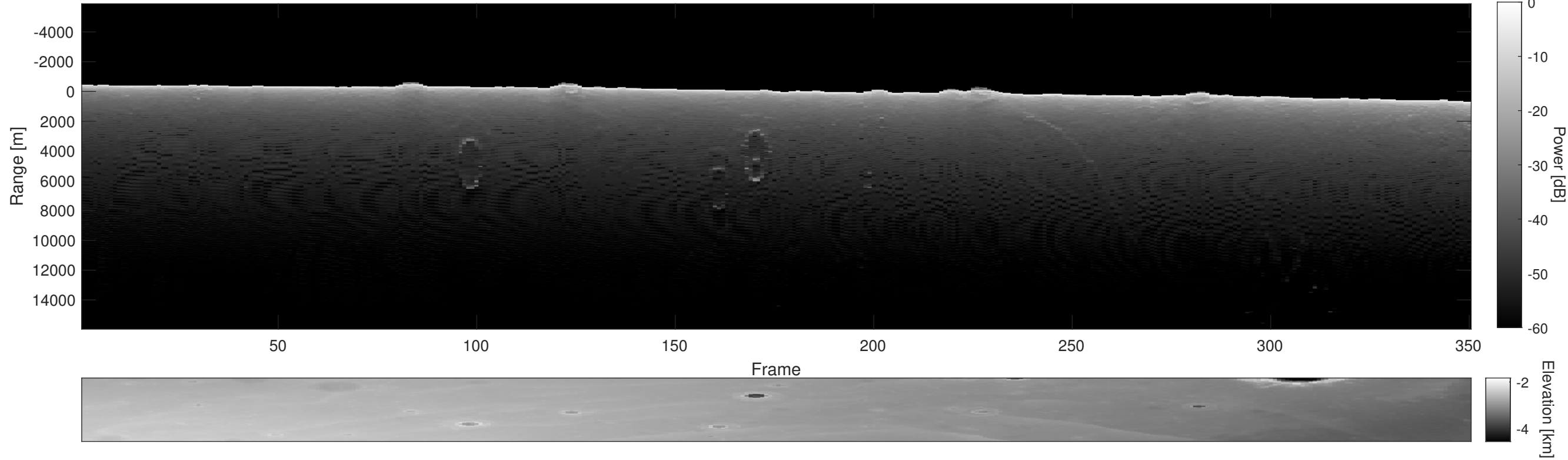
Orbit 16050, Depth-Corrected Cluttergram
