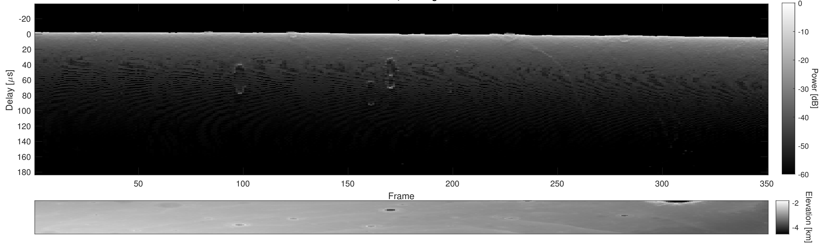
Orbit 16050, Cluttergram
