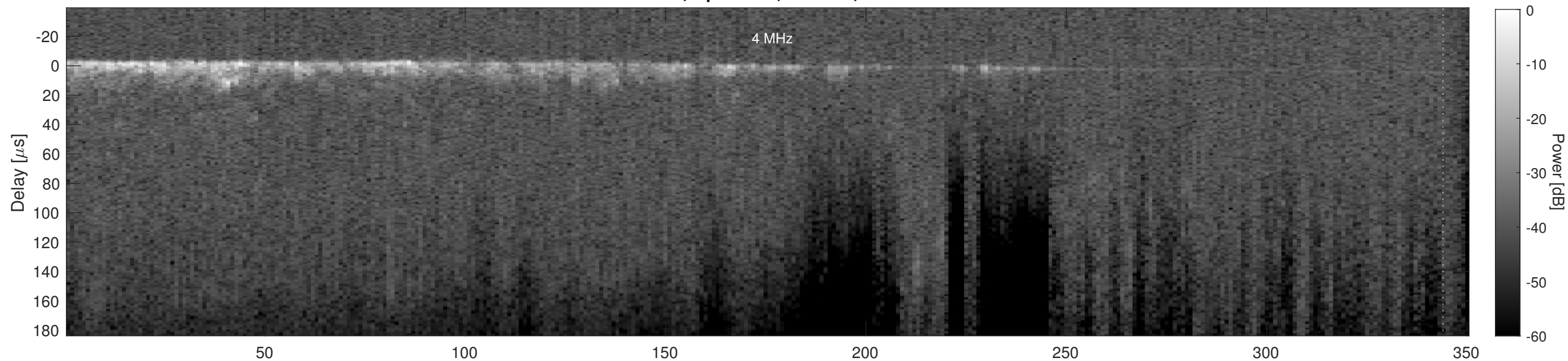
Orbit 16050, Cluttergram
