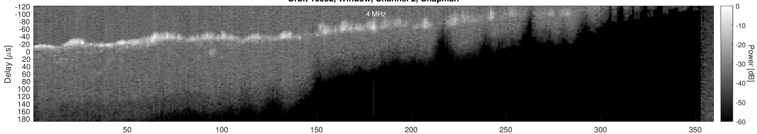
Orbit 16052, Window, Channel 2, Optimized
