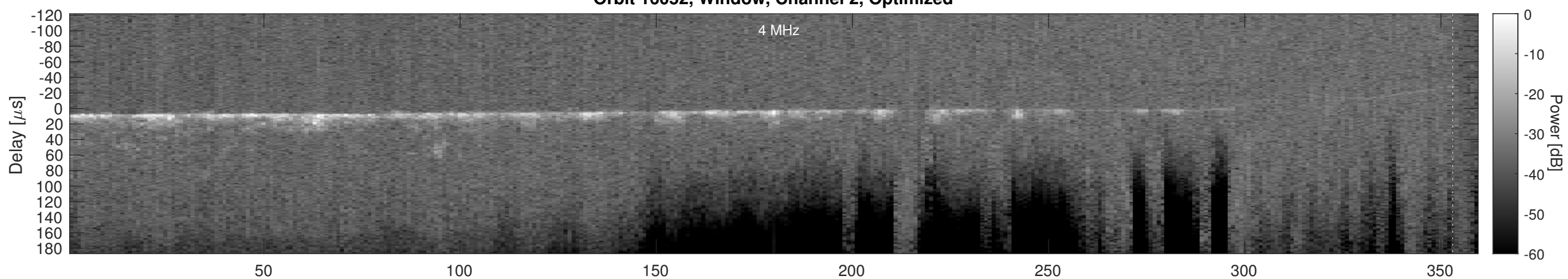
Orbit 16052, Cluttergram
