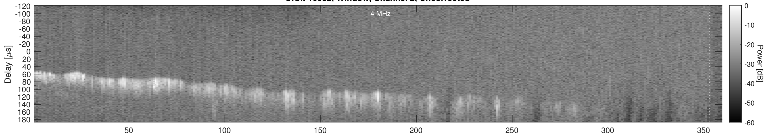
Orbit 16052, Window, Channel 2, Chapman
