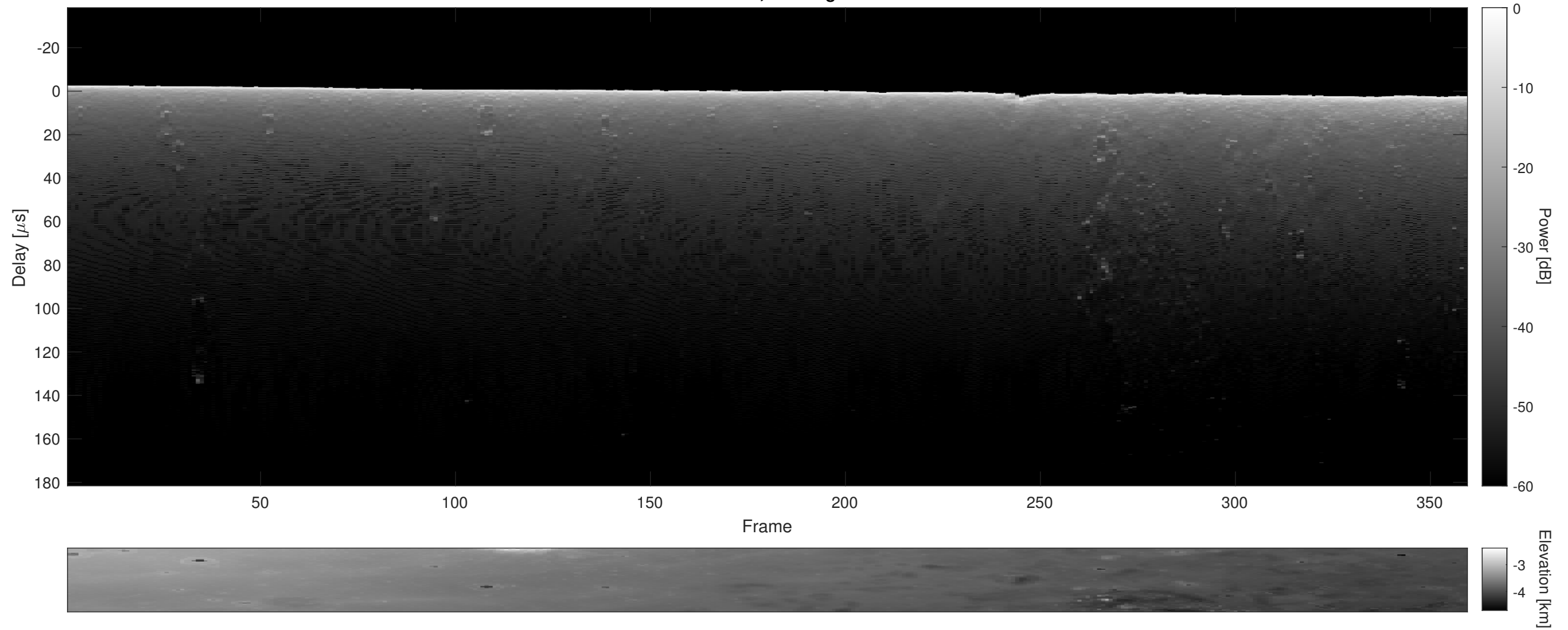
Orbit 16055, Cluttergram
