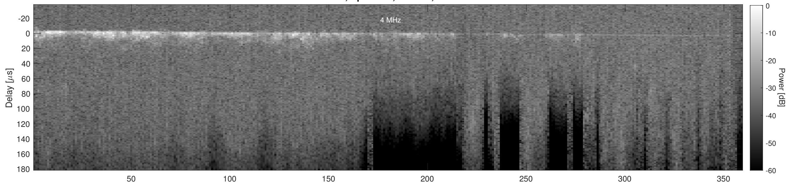
Orbit 16055, Cluttergram
