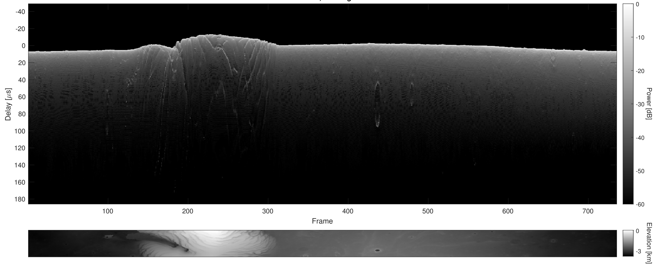
Orbit 16103, Cluttergram
