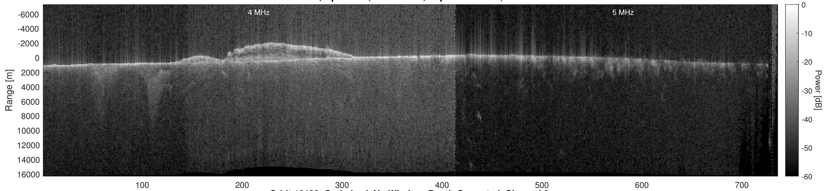
Orbit 16103, Optimized, No Window, Depth-Corrected, Channel 2
