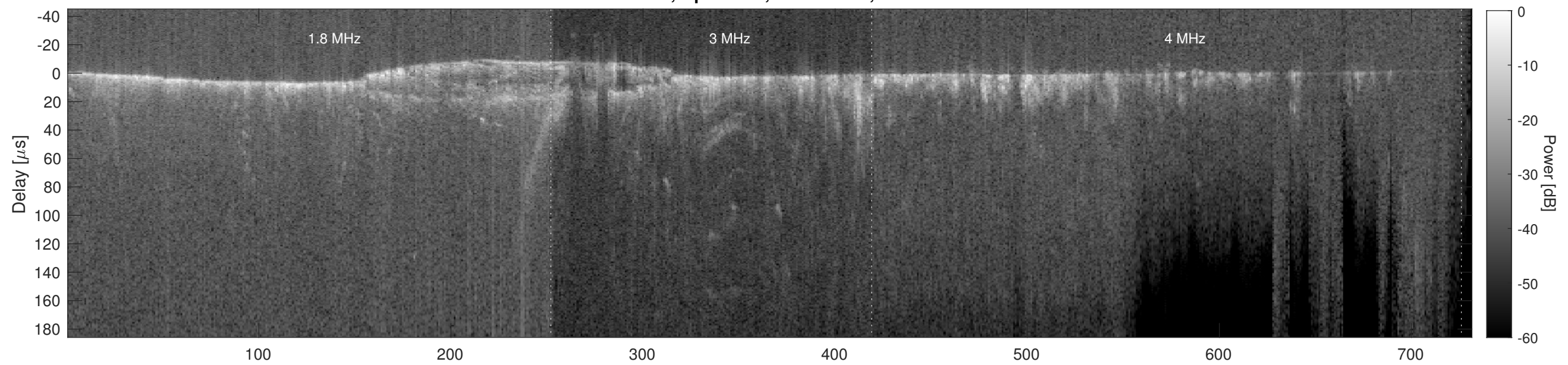
Orbit 16107, Cluttergram
