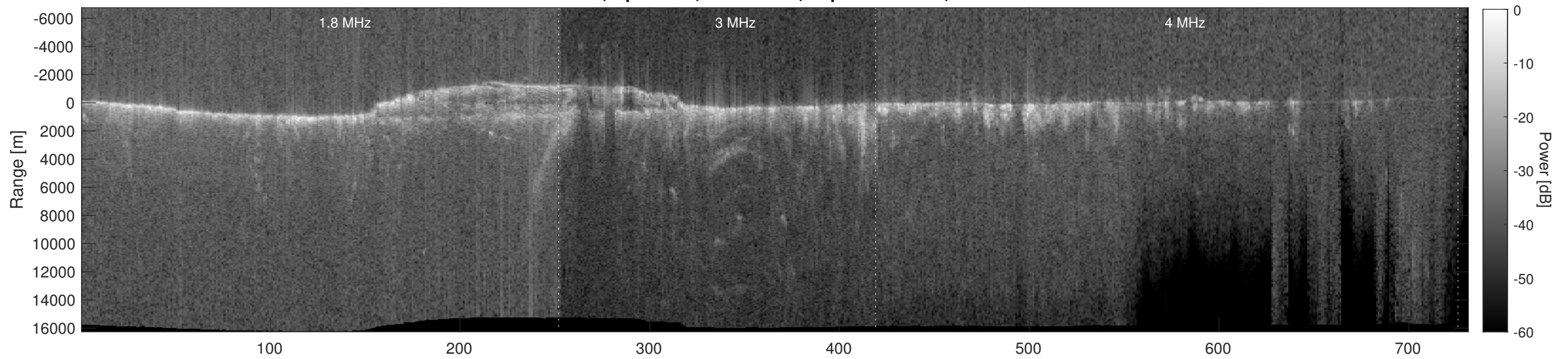
Orbit 16107, Depth-Corrected Cluttergram
