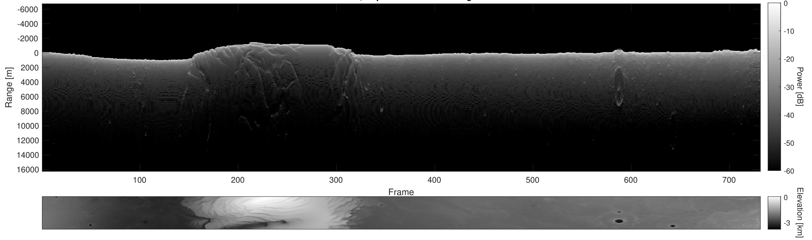
Orbit 16107, Depth-Corrected Cluttergram
