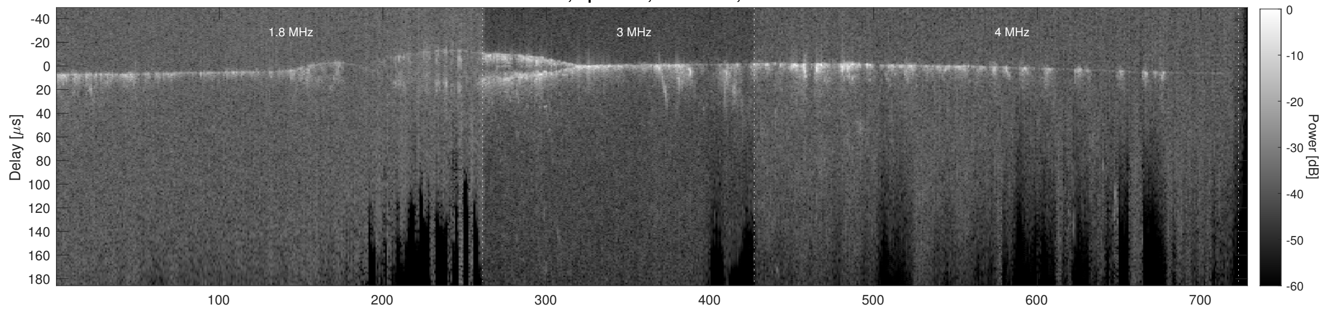
Orbit 16110, Cluttergram
