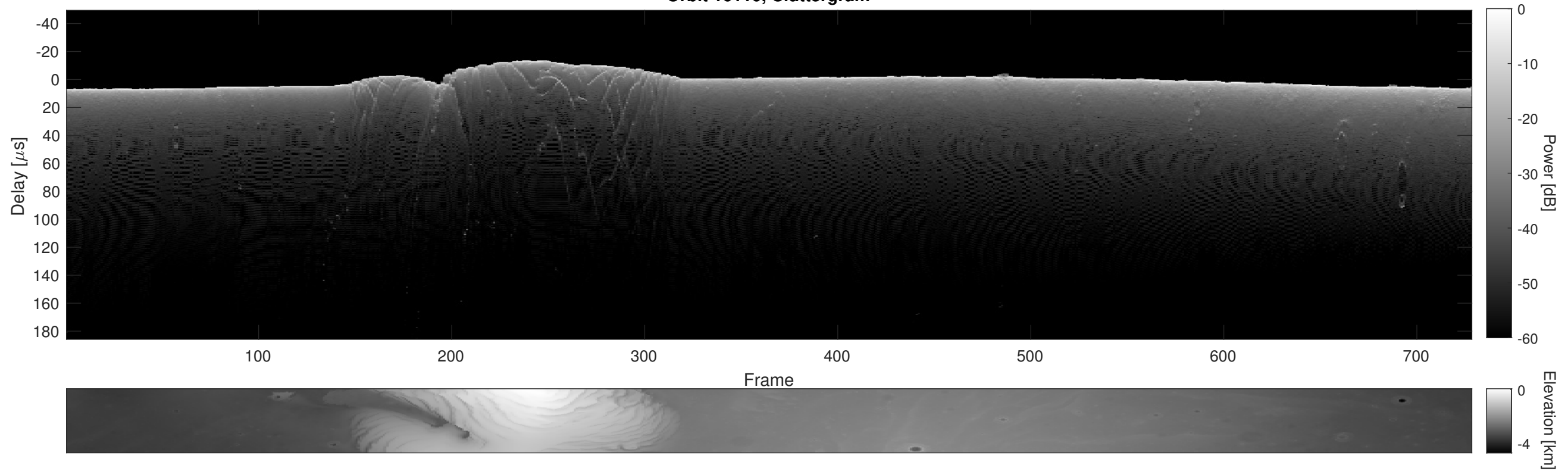
Orbit 16110, Cluttergram
