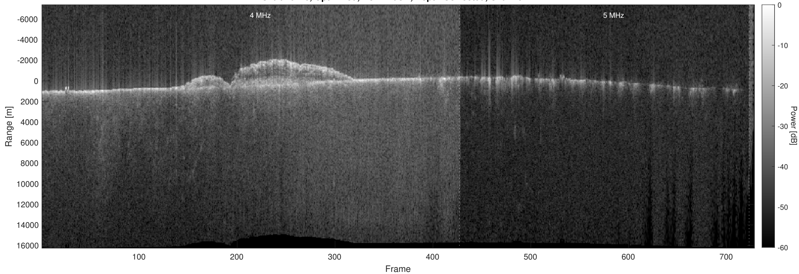
Orbit 16110, Optimized, No Window, Depth-Corrected, Channel 2
