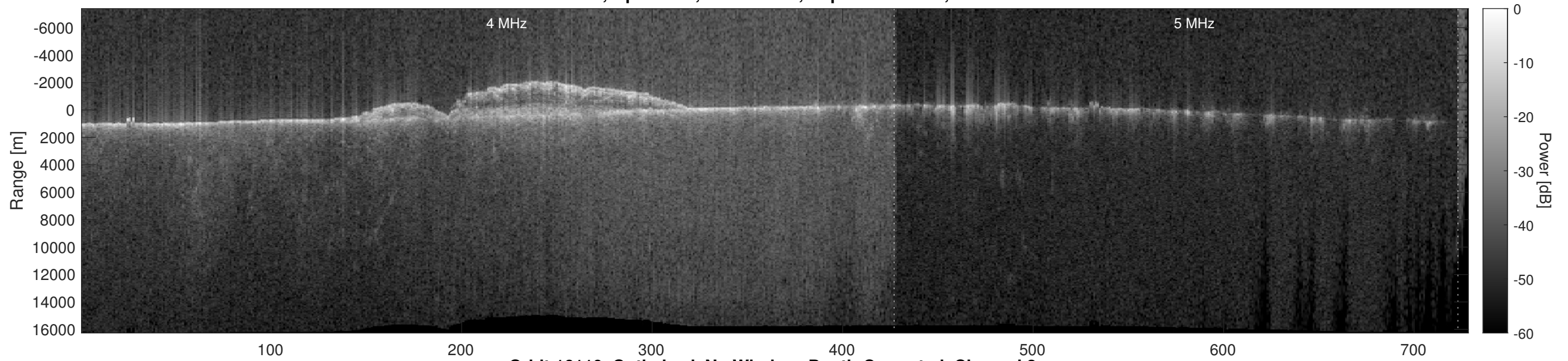
Orbit 16110, Optimized, No Window, Depth-Corrected, Channel 2
