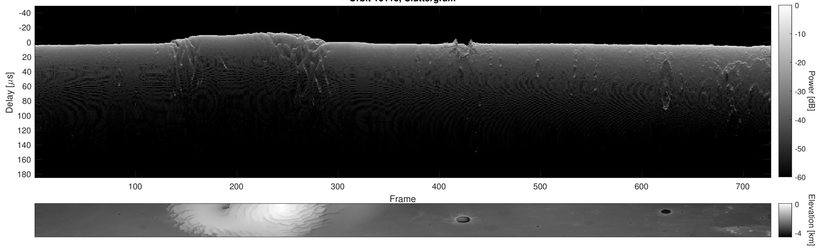
Orbit 16113, Cluttergram
