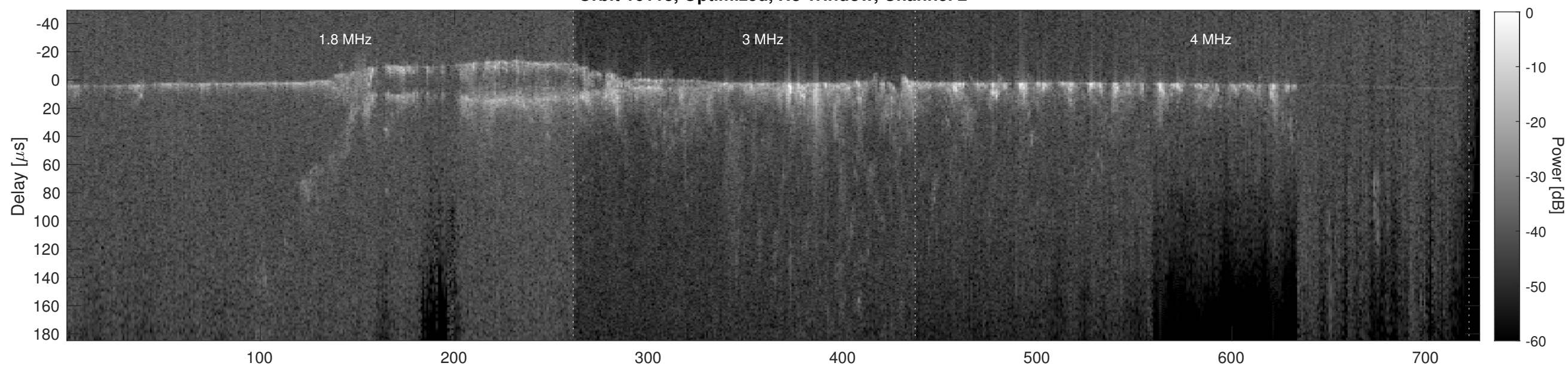
Orbit 16113, Cluttergram
