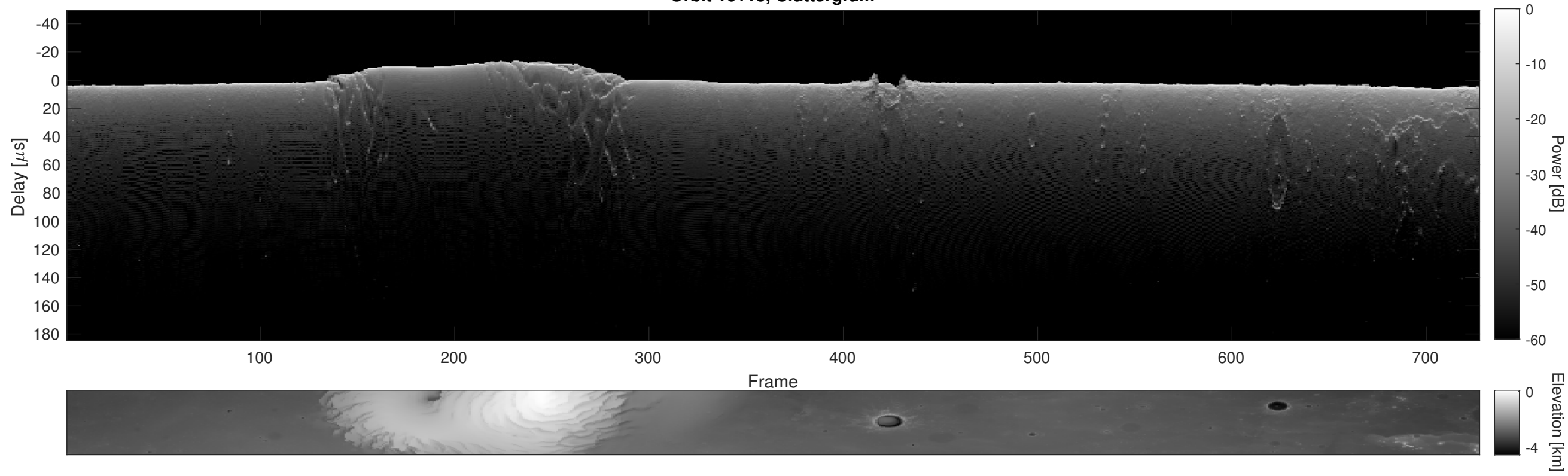
Orbit 16113, Cluttergram
