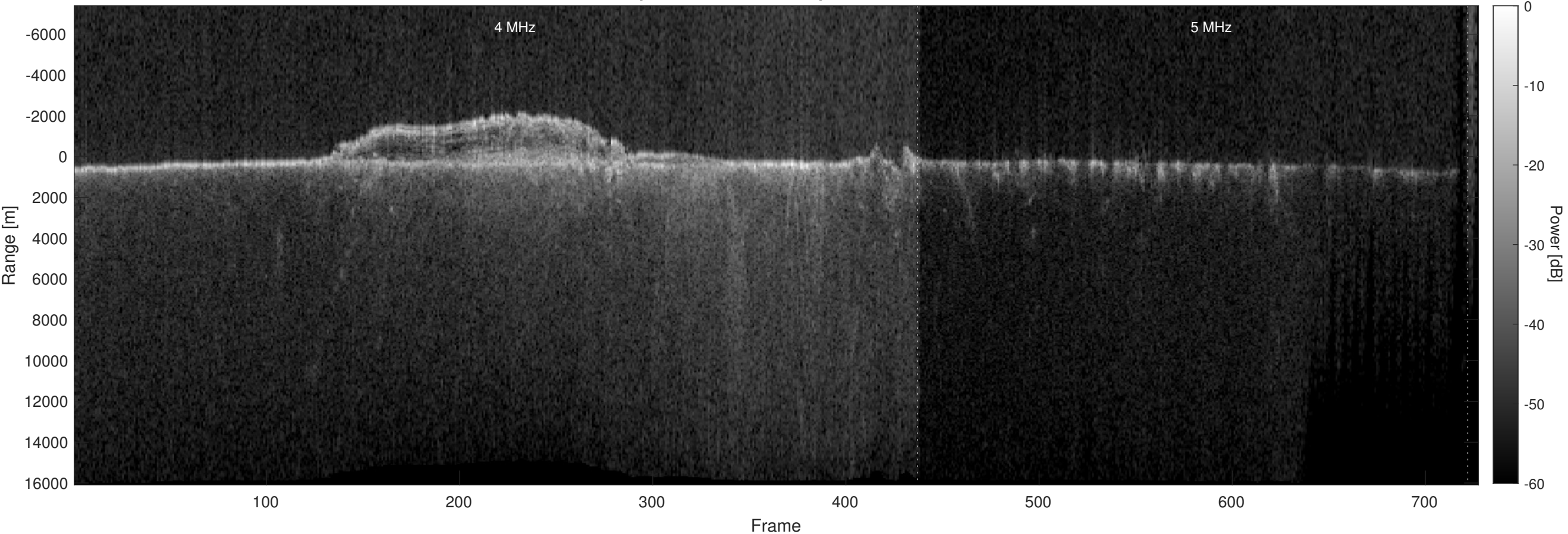
Orbit 16113, Optimized, Window, Depth-Corrected, Channel 2
