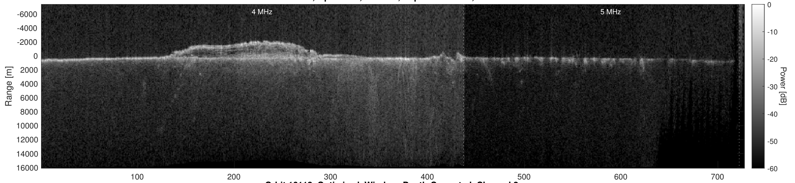
Orbit 16113, Optimized, Window, Depth-Corrected, Channel 2
