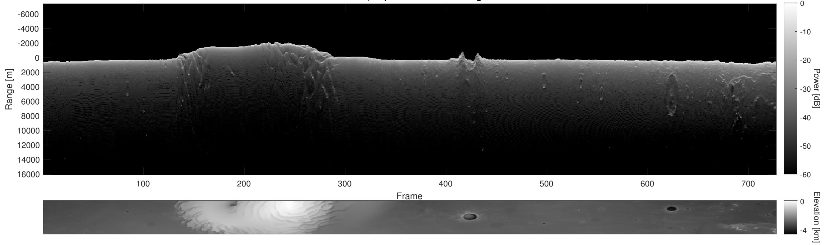
Orbit 16113, Depth-Corrected Cluttergram
