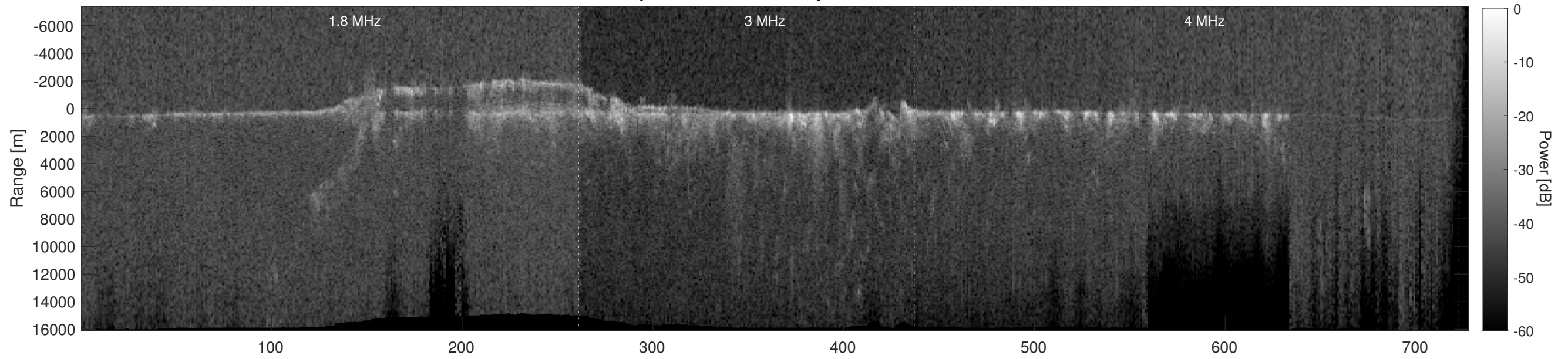
Orbit 16113, Depth-Corrected Cluttergram
