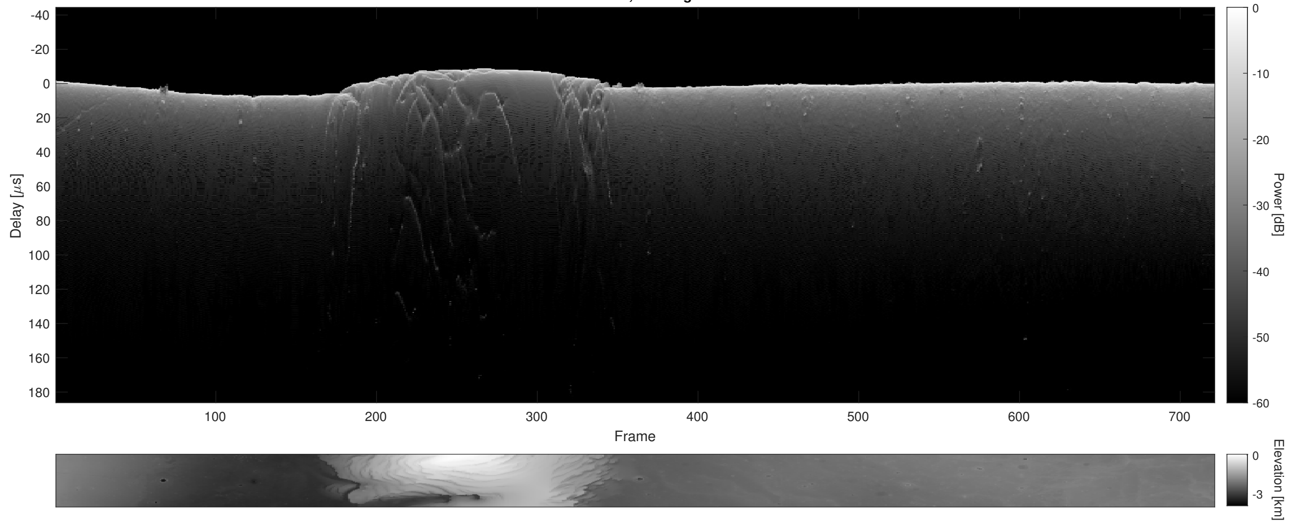
Orbit 16121, Cluttergram
