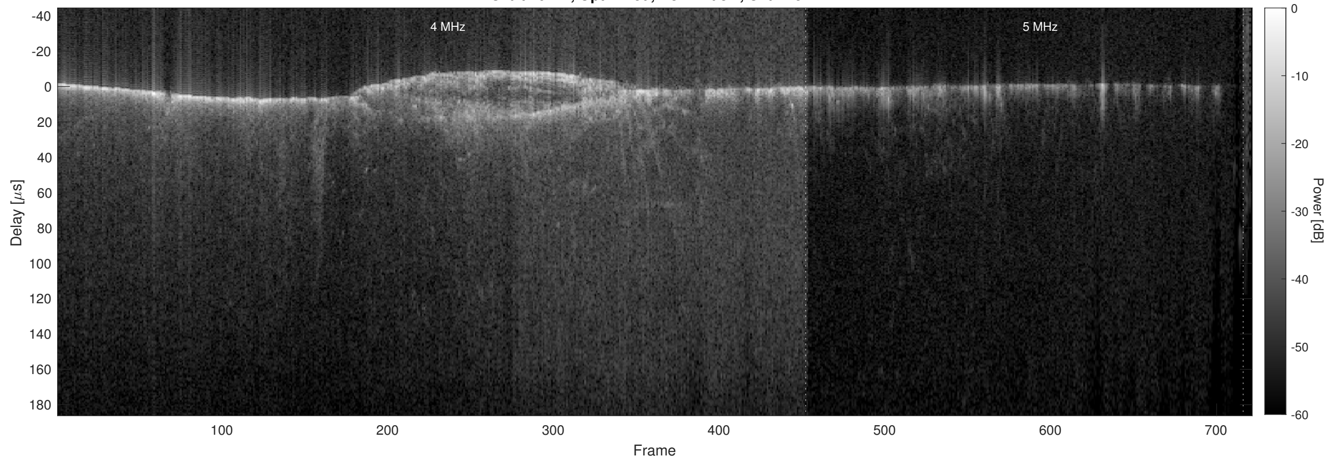
Orbit 16121, Optimized, No Window, Channel 2
