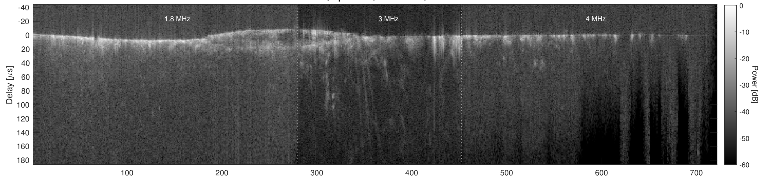
Orbit 16121, Cluttergram
