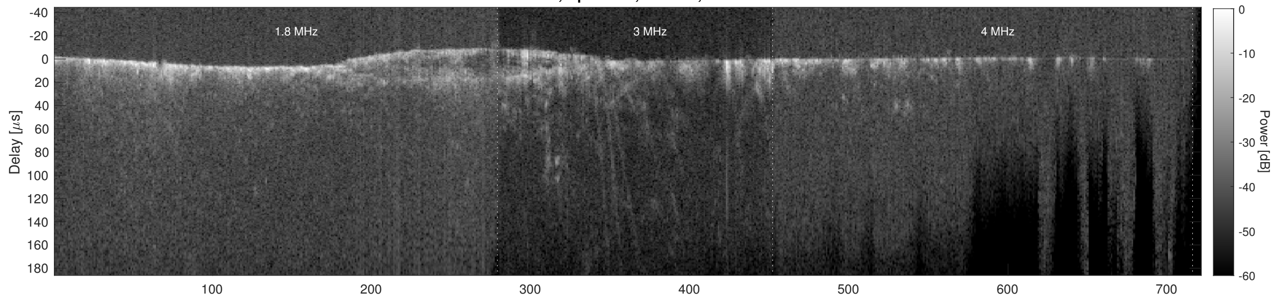
Orbit 16121, Cluttergram
