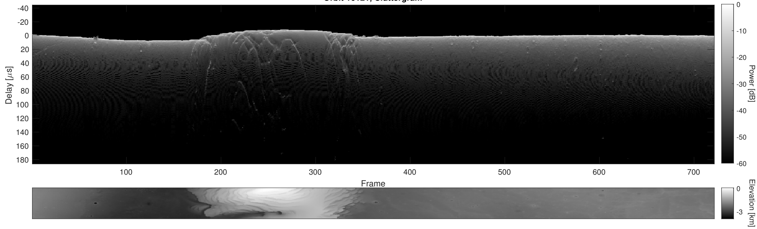
Orbit 16121, Cluttergram
