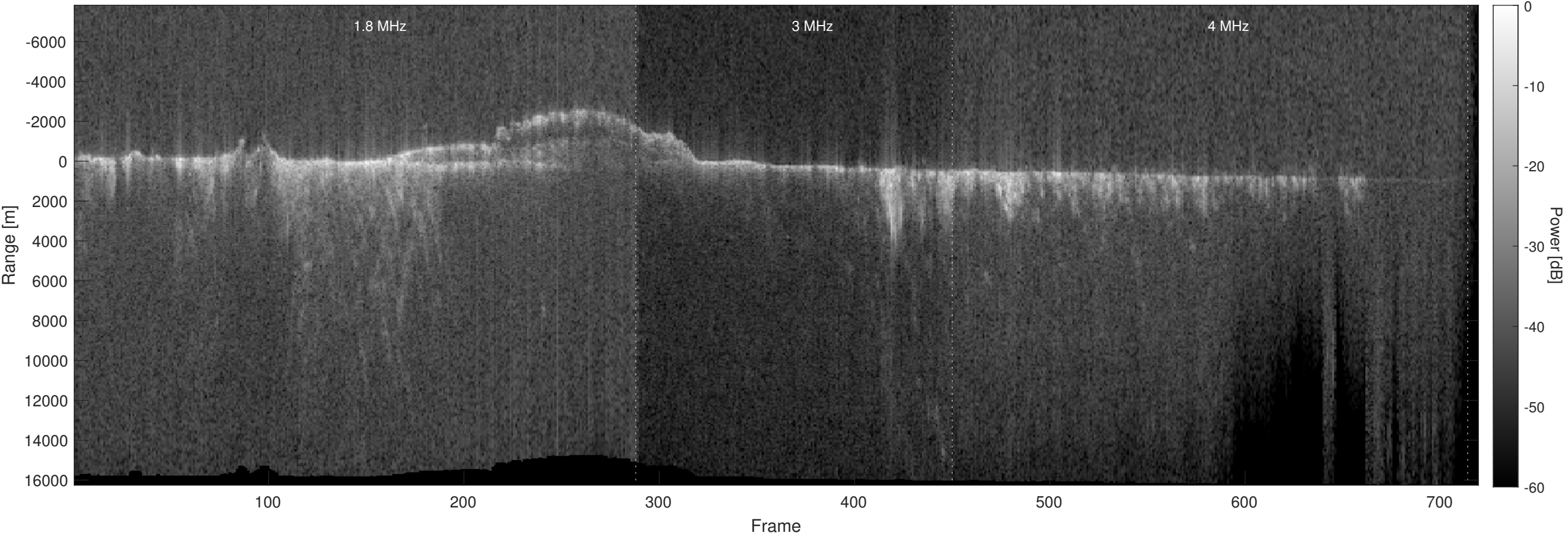
Orbit 16122, Optimized, No Window, Depth-Corrected, Channel 2
