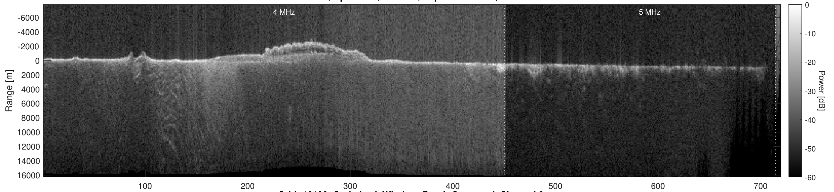
Orbit 16122, Optimized, Window, Depth-Corrected, Channel 2
