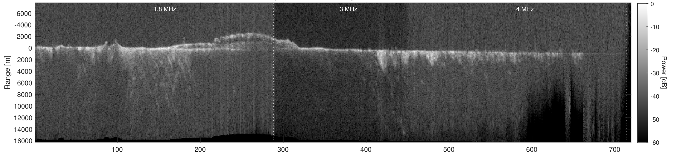
Orbit 16122, Depth-Corrected Cluttergram
