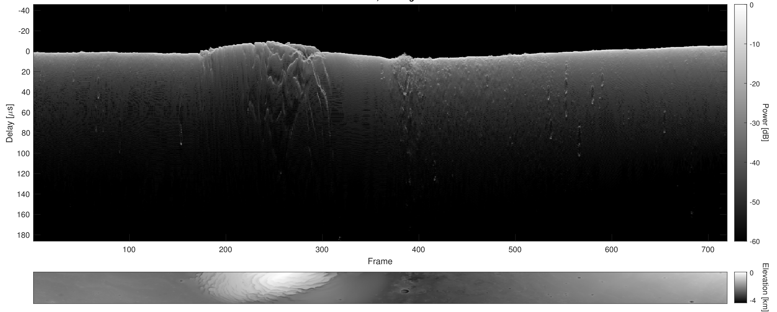
Orbit 16123, Cluttergram
