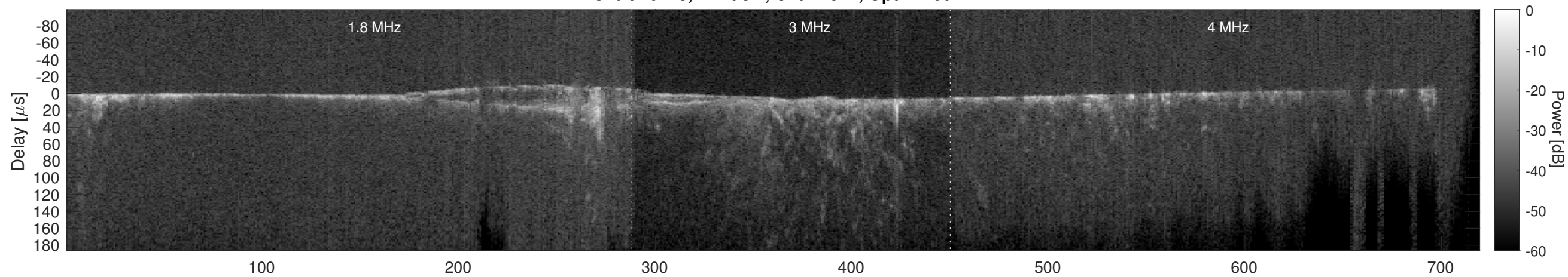
Orbit 16123, Cluttergram
