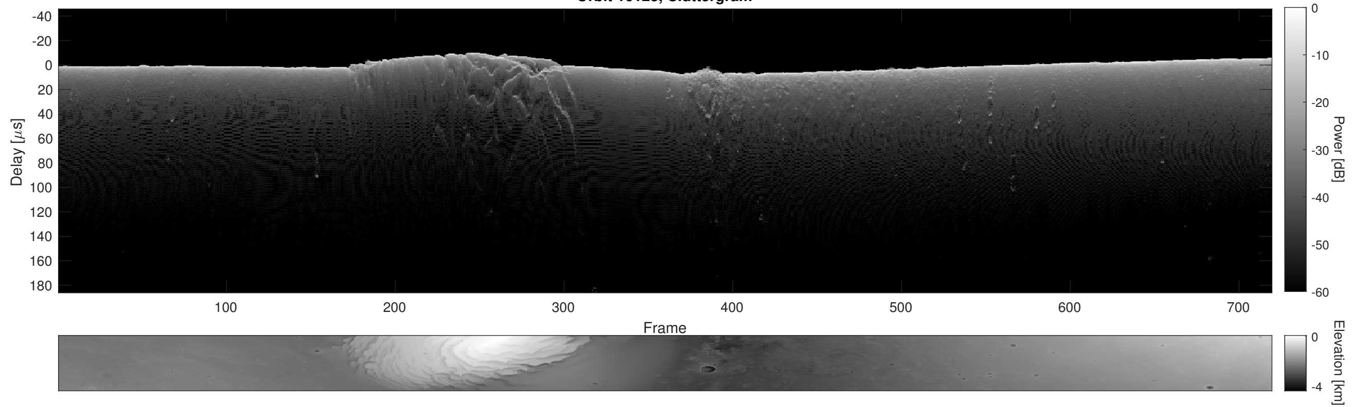
Orbit 16123, Cluttergram
