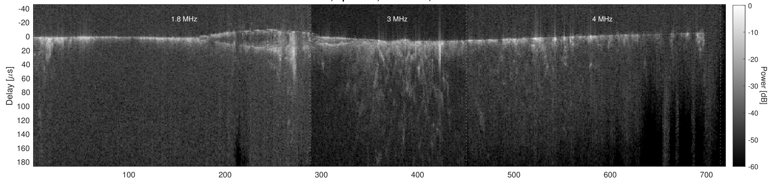
Orbit 16123, Cluttergram
