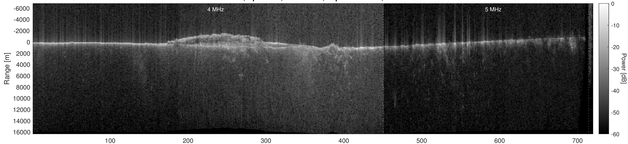
Orbit 16123, Optimized, No Window, Depth-Corrected, Channel 2
