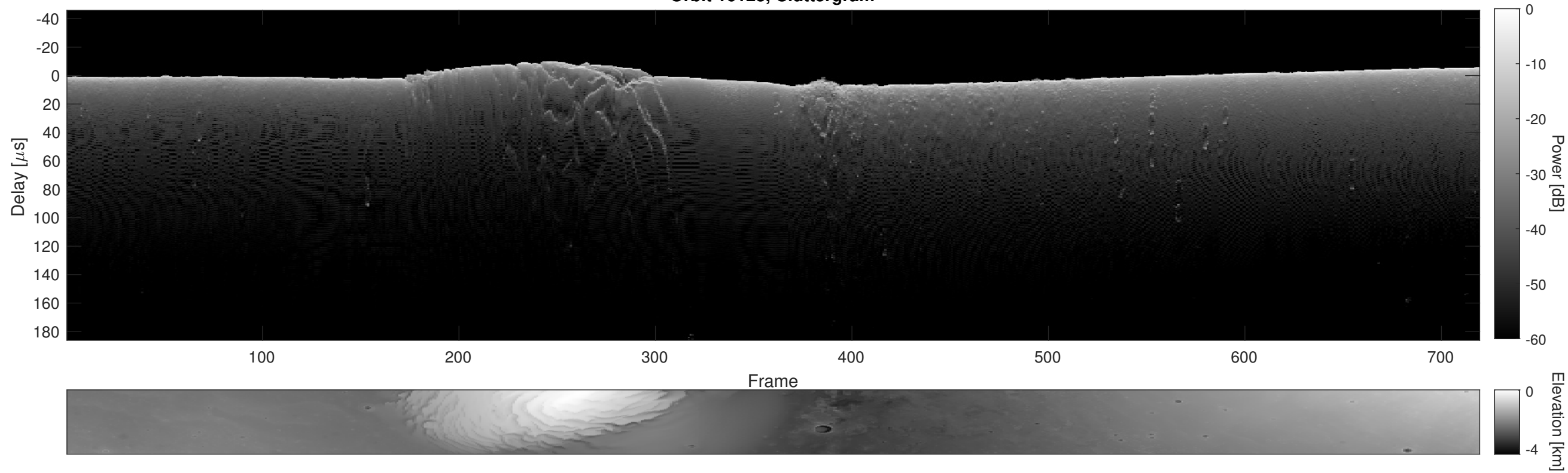
Orbit 16123, Cluttergram
