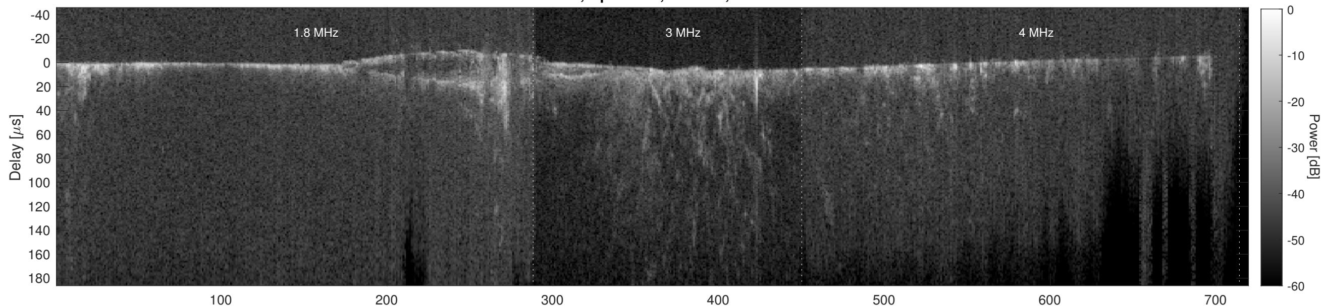
Orbit 16123, Cluttergram
