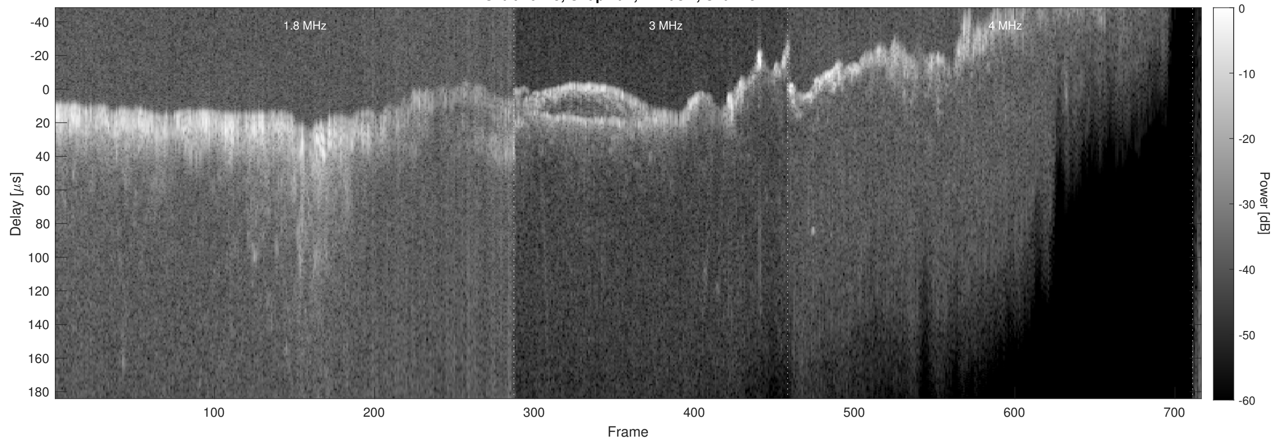
Orbit 16125, Chapman, Window, Channel 2
