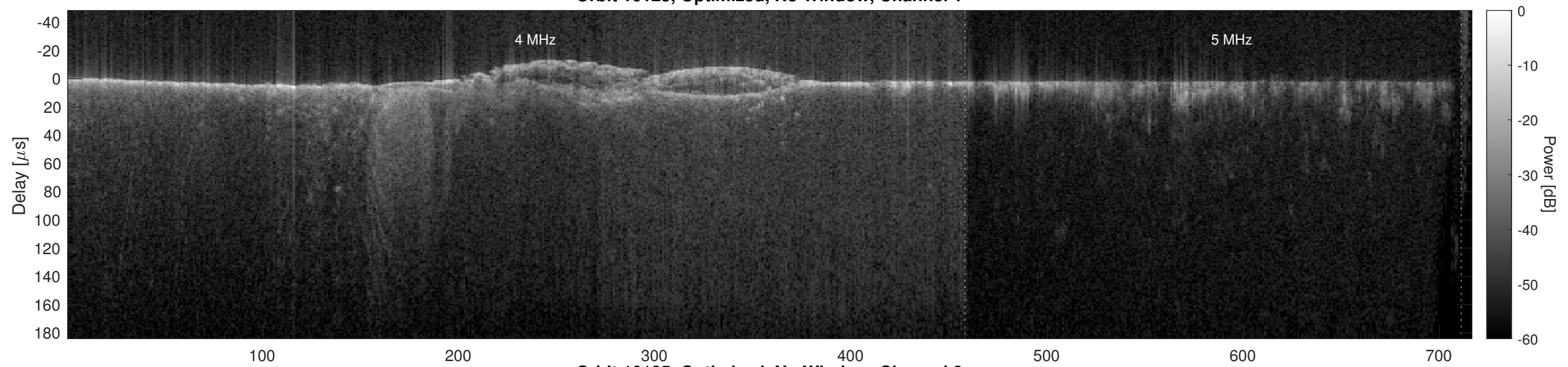
Orbit 16125, Optimized, No Window, Channel 2
