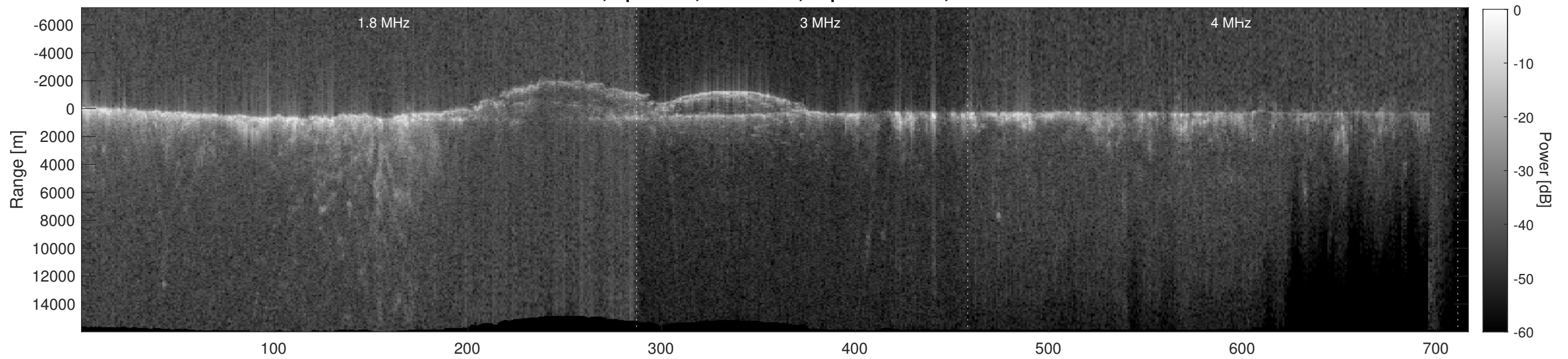
Orbit 16125, Depth-Corrected Cluttergram
