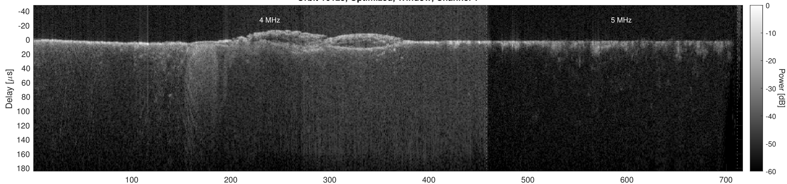
Orbit 16125, Optimized, Window, Channel 2
