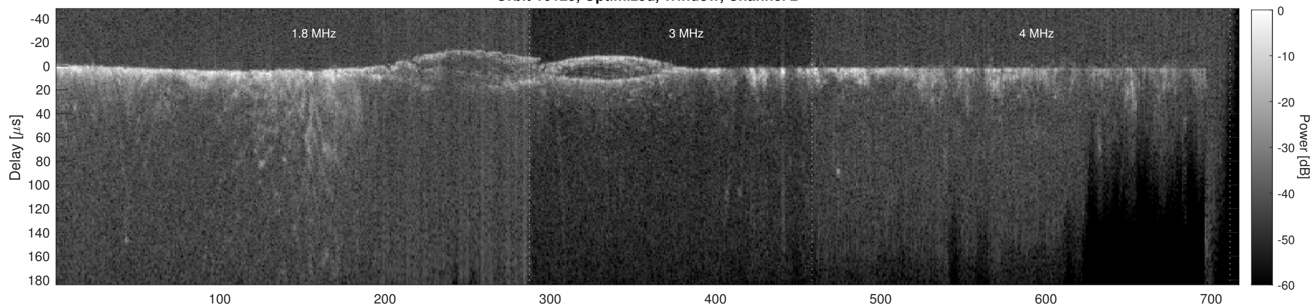
Orbit 16125, Cluttergram
