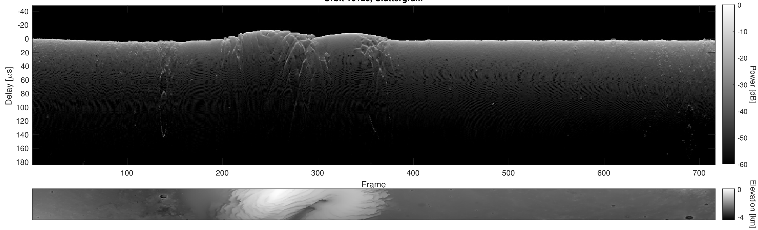
Orbit 16125, Cluttergram
