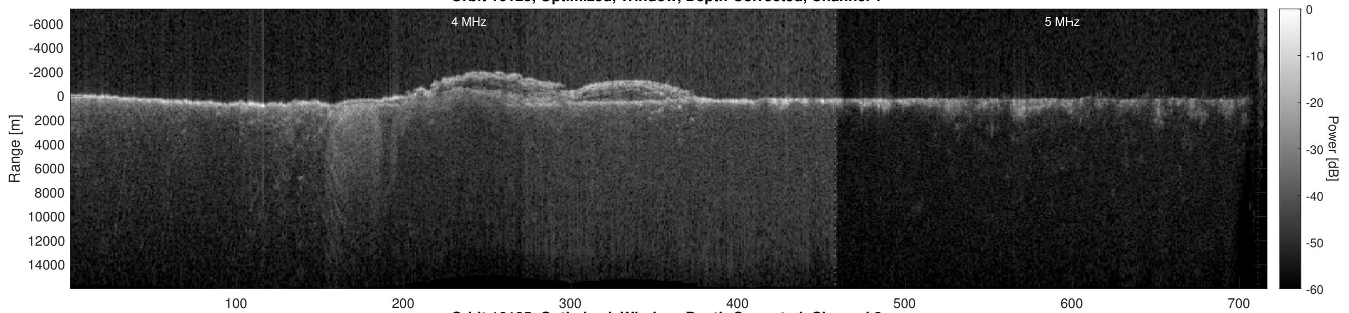
Orbit 16125, Optimized, Window, Depth-Corrected, Channel 2
