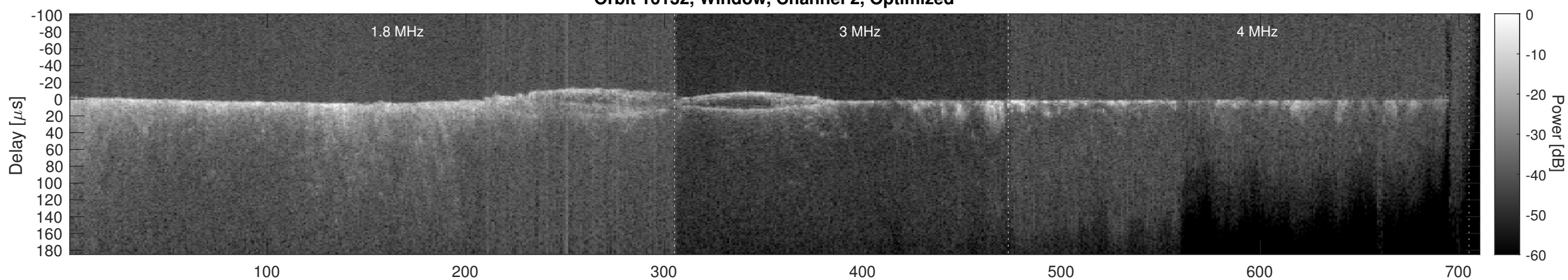
Orbit 16132, Cluttergram
