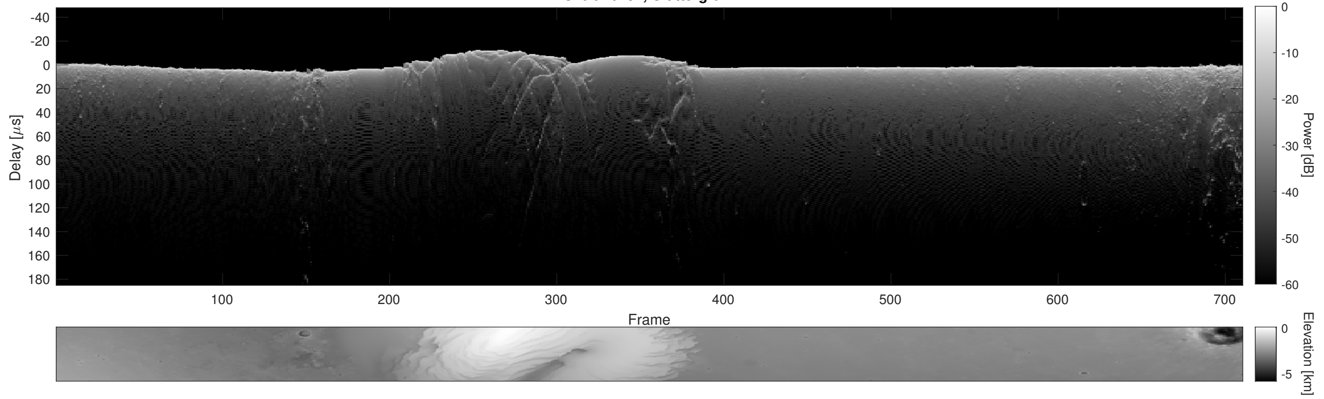
Orbit 16132, Cluttergram
