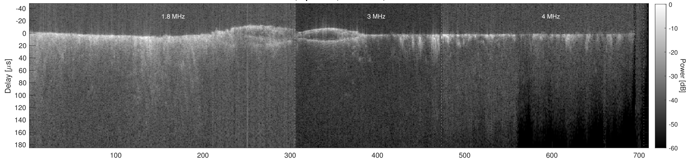
Orbit 16132, Cluttergram
