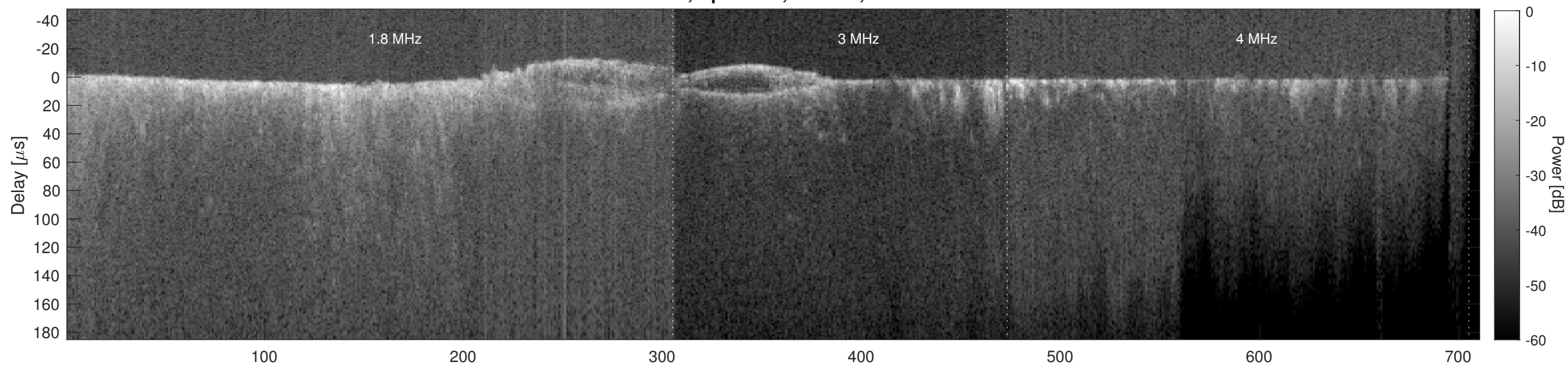
Orbit 16132, Cluttergram
