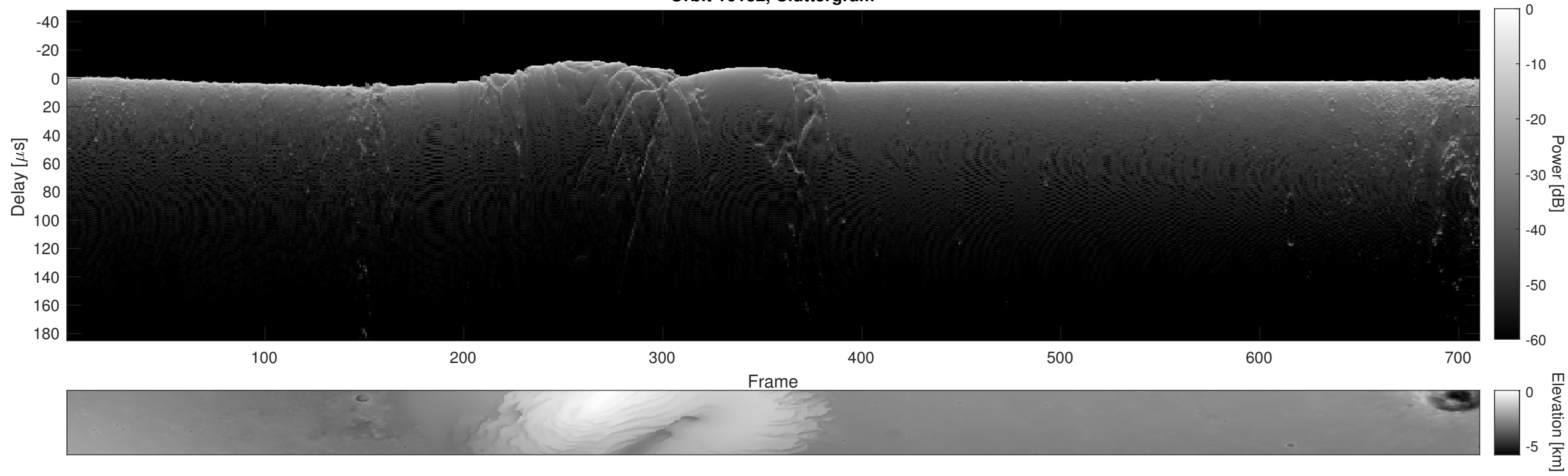
Orbit 16132, Cluttergram
